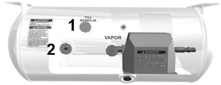
1-Propane fill valve; 2-Propane gauge ASME tank
